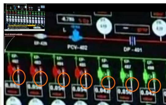
Figure 7: Control loops (highlighted in orange) in a SCADA display from Natanz indicate that the stage exhaust valves are controlled in a closed loop by dedicated pressure controllers
